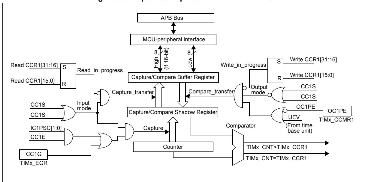
Figure 30. Capture/compare channel 1 main circuit
